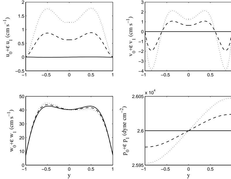
Figure 2. Amplitude of the unsteady solution \chi_0 + \varepsilon \hat{\chi}_1 for \varepsilon = 0 (continuous line), \varepsilon = 0.05 (dashed line) and \varepsilon = 0.1 (dotted line) along [-1, 1] .
