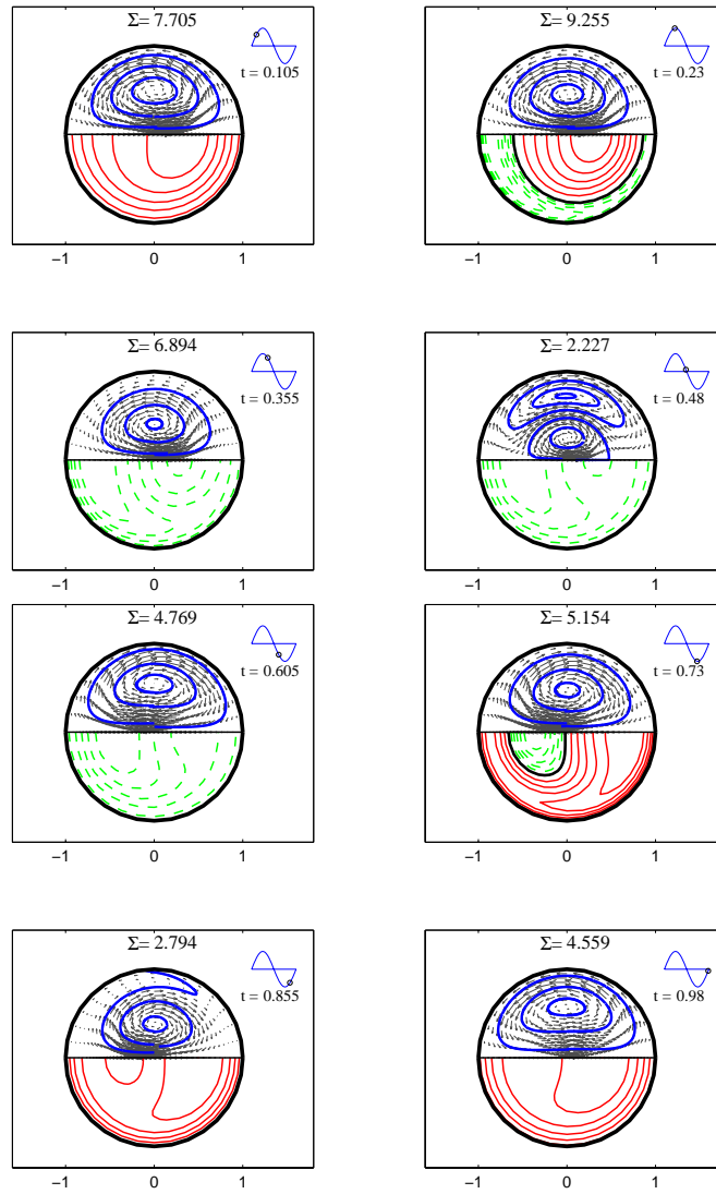
Figure 3. Streamlines and secondary flow (above) and contour equispaced lines for axial velocity (below - continuous lines indicate positive levels, dashed lines negative levels, bold line zero levels) at eight times in a period at z = 0 . The plot refers to the steady state solution summed up to unsteady solution \bar{\chi} + \bar{\chi}e^{i(\omega t - kz)} , with \varepsilon = 0.1 . A double vortex develops at the end of each half-cycle in correspondence of a small \Sigma .
