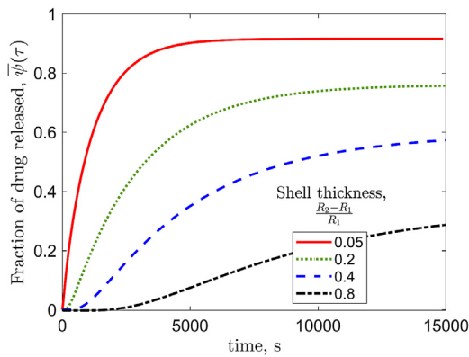
Fig. 10. Effect of shell thickness: \bar{\psi}(\tau) as a function of dimensional time for multiple values of shell thickness R_2 - R_1 for a fixed core radius, R_1 = 1.5 mm. Other parameters are D_1 = 30 \times 10^{-11} \text{ m}^2\text{s}^{-1} ; D_2 = 5 \times 10^{-11} \text{ m}^2\text{s}^{-1} ; h = 3.17 \times 10^{-5} \text{ ms}^{-1} ; \sigma_1 = 1 ; \beta_1 = \beta_2 = 8.06 \times 10^{-5} \text{ s}^{-1} .
