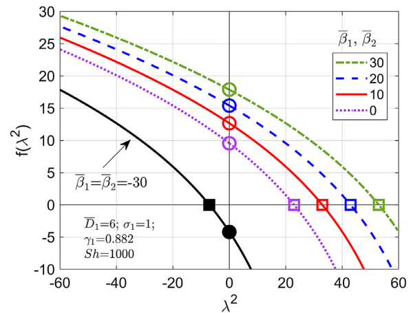
Fig. 2. Eigenfunction plot in both real and imaginary spaces to illustrate the impact of Damköhler numbers on the nature of eigenvalues. Plot parameters are \bar{D}_1 = 6 ; \sigma_1 = 1 ; \gamma_1 = 0.882 ; Sh = 1000 . Square markers indicate the first eigenvalue. Circular markers indicate the value of the eigenfunction at the transition between real and imaginary eigenvalues, \lambda^2 = 0 . A case of negative Damköhler number is also shown for illustration of a case of imaginary eigenvalues.
