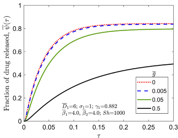
Fig. 11. Effect of thin outer coating: \bar{\psi}(\tau) as a function of \tau for multiple values of \bar{g} . Other problem parameters are \bar{D}_1 = 6 ; \sigma_1 = 1 ; \gamma_1 = 0.882 ; \bar{\beta}_1 = \bar{\beta}_2 = 4 ; Sh = 1000 .
